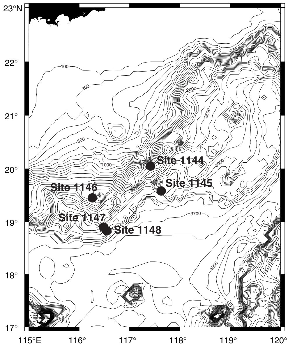
ODP Leg 184 Site Map (Part C) Sites 1144–1148 (northern area)
