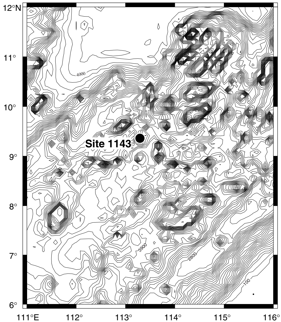
ODP Leg 184 Site Map (Part B) Site 1143 (southern area)
